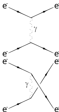
FIGURE 1. Feynman diagrams for Möller scattering t- and u-channels, top and bottom respectively
